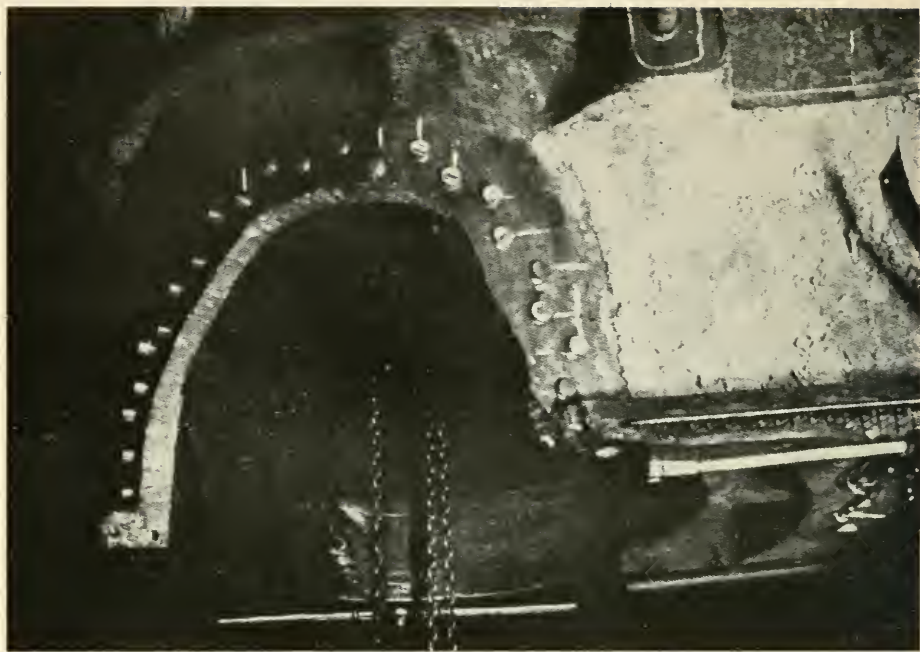
"PRINZESS IRENE" DAMAGED H. P. CYLINDER, READY FOR INSERT, PREPARATORY TO WELDING
